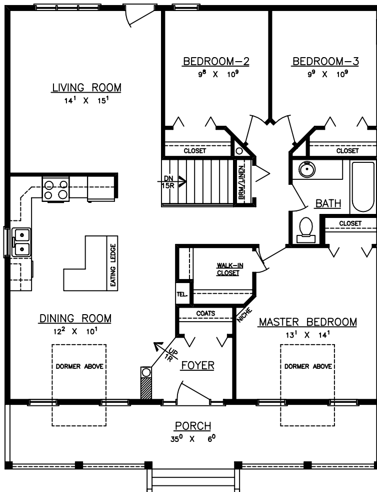
FLOOR PLAN
